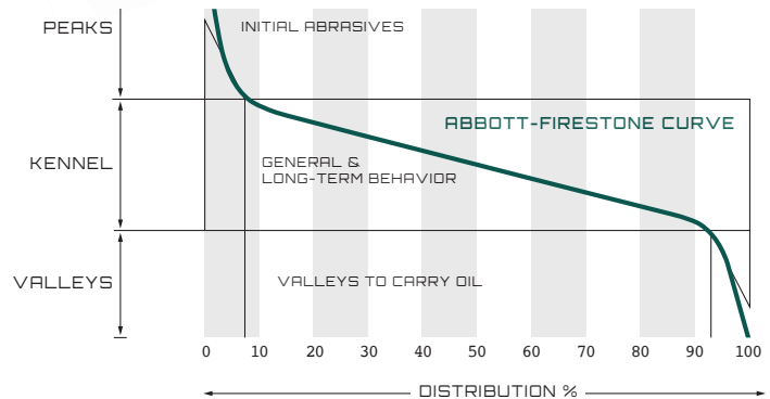
ABBOTT-FIRESTONE SURFACE PARAMETERS
