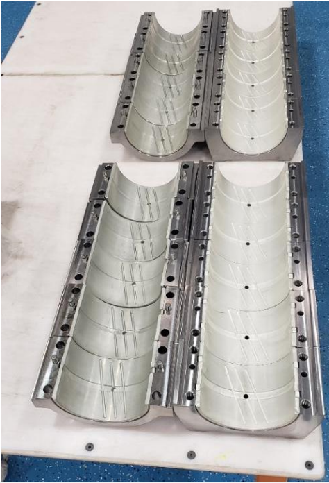
Pic 3 Broken Apart Before Crankshaft Assy
